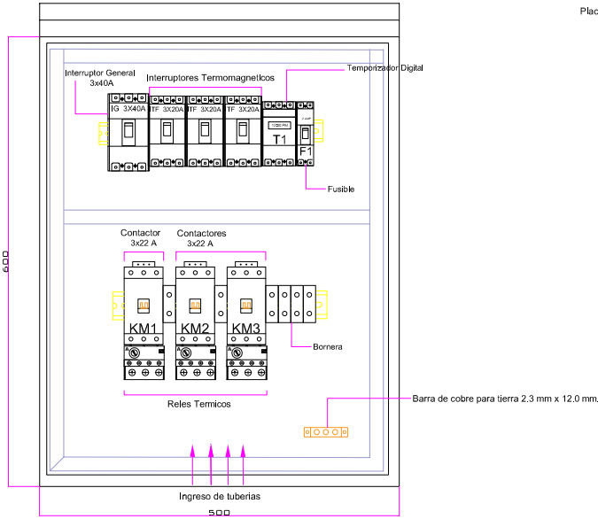
VISTA FRONTAL INTERIOR
