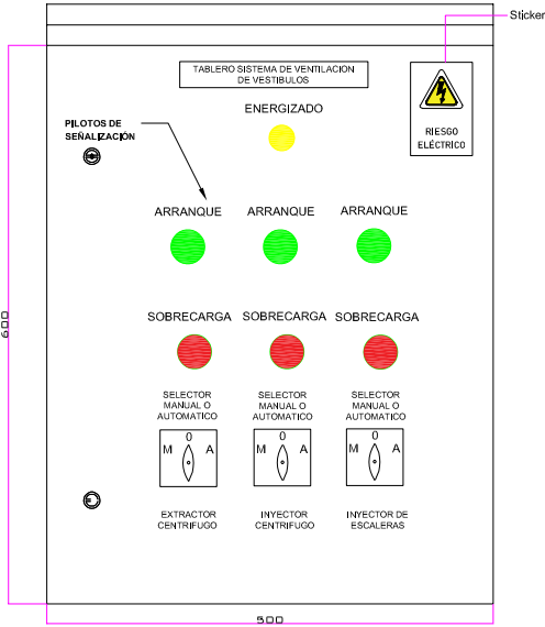
VISTA FRONTAL EXTERIOR
